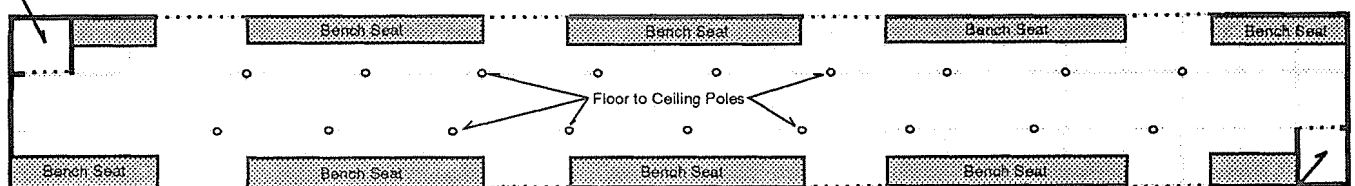
Motorman's Cab
