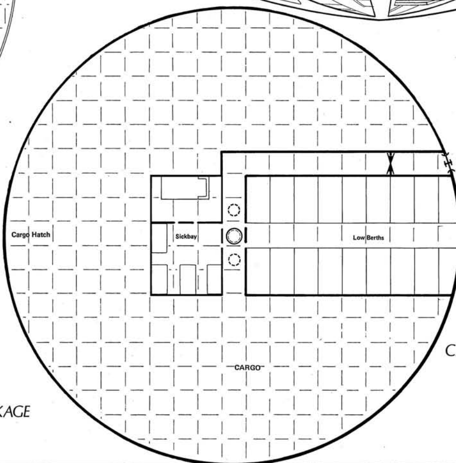
MAIN DECK
