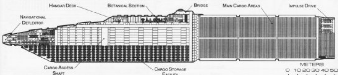
CROSS SECTION
