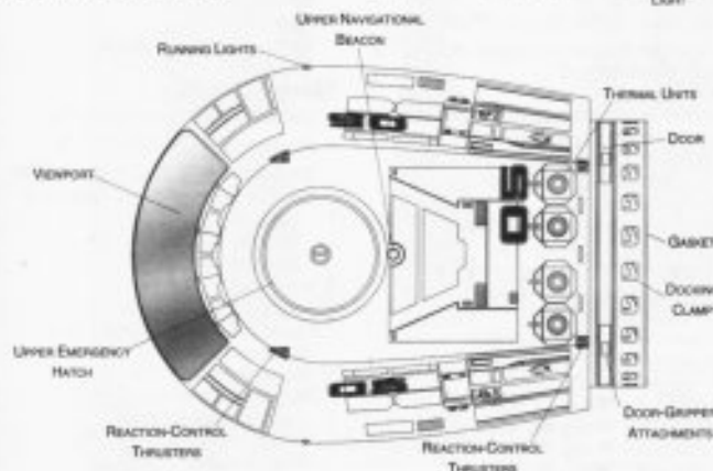
TOP PROFILE
