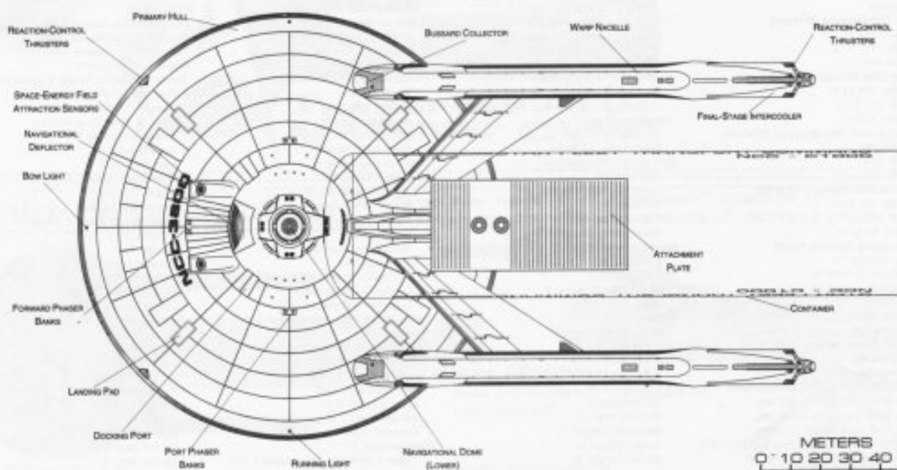
BOTTOM PROFILE
