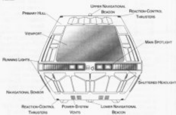
FRONT PROFILE
