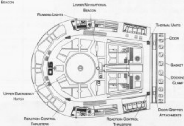
BOTTOM PROFILE
