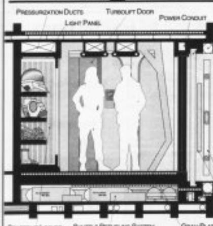
CROSS SECTION
