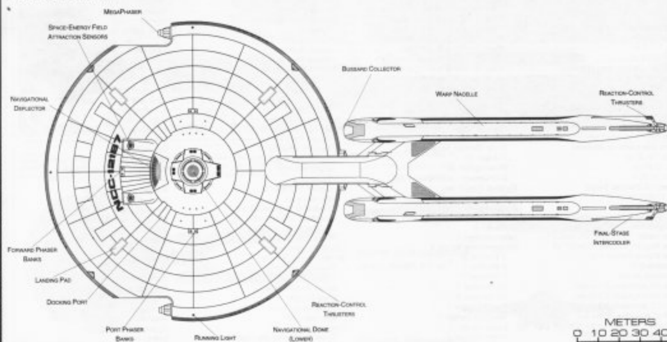
BOTTOM PROFILE
