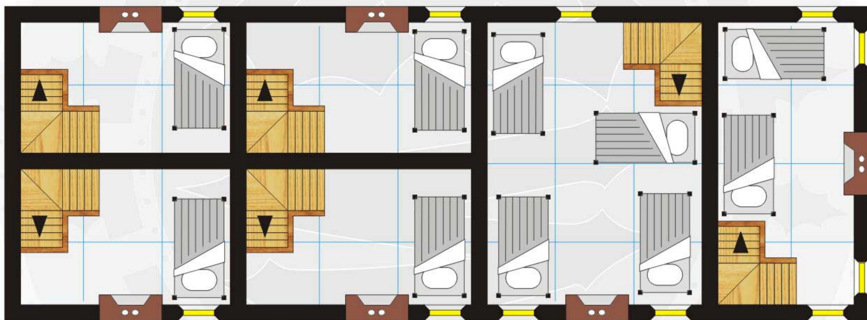
Second Floor
