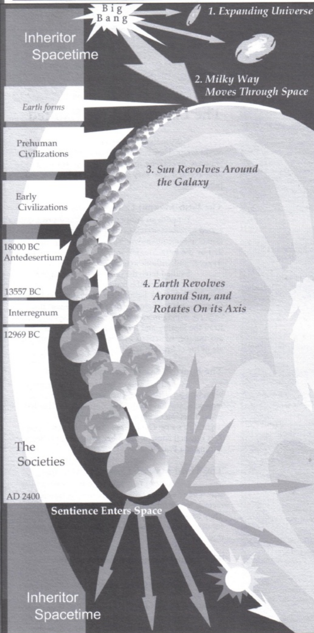
SPACETIME MAP OF EARTH — Not to Scale.
